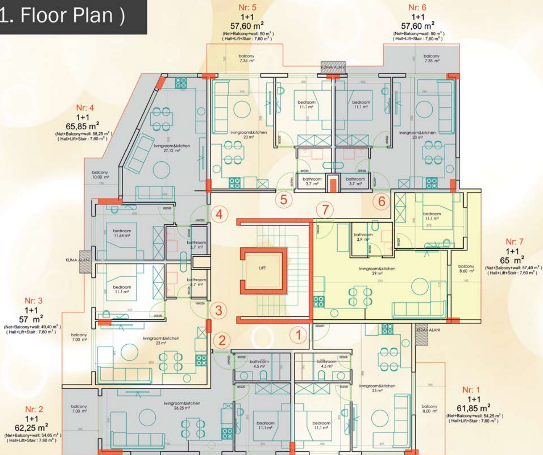
1. FLOOR PLAN
