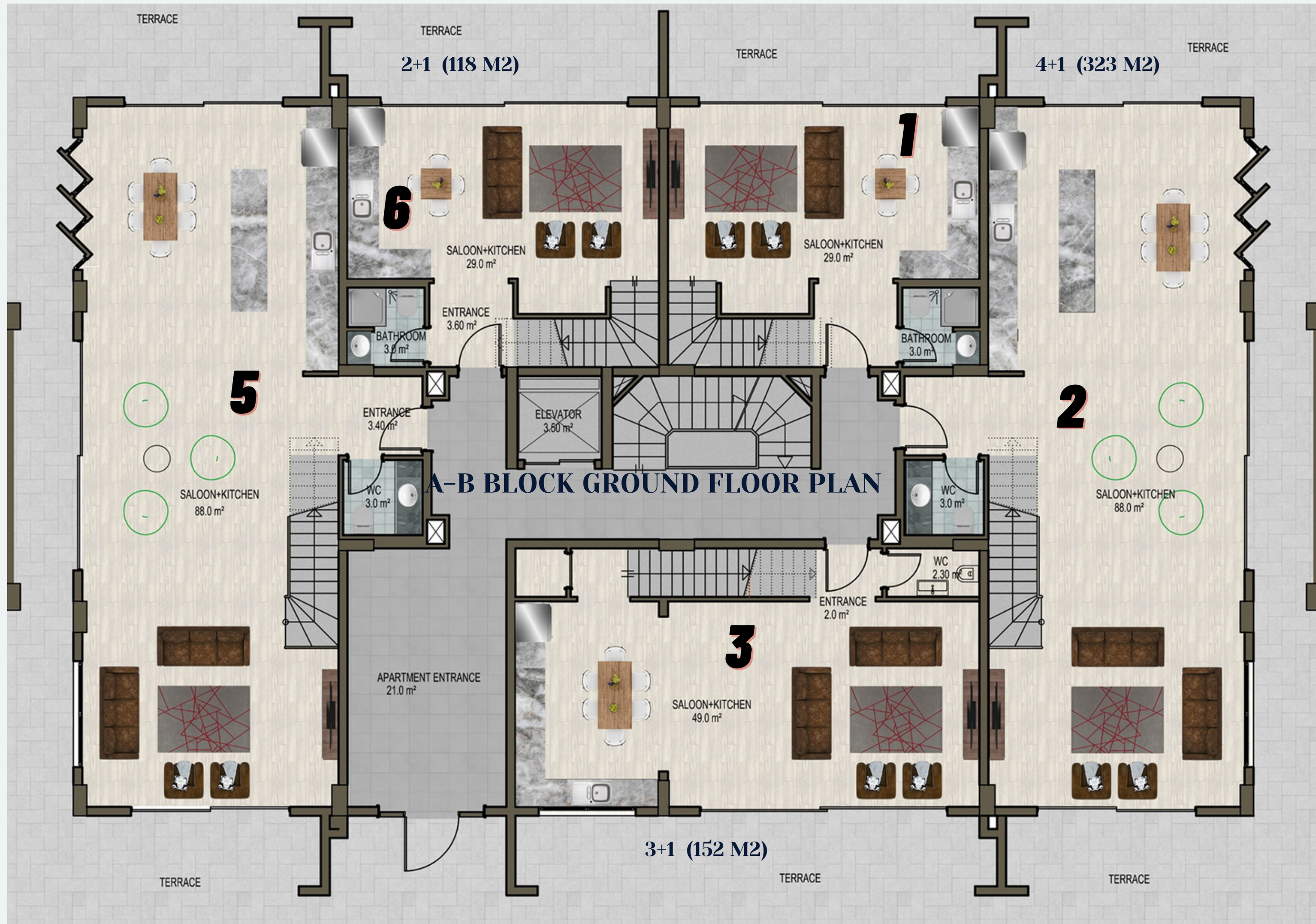
A VE B ZEMIN KATPLANI
